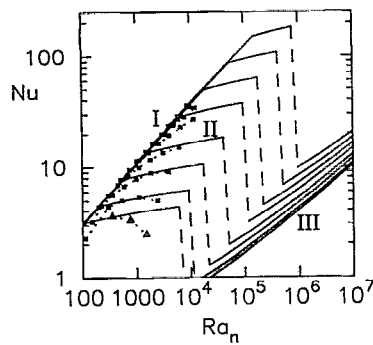
FIG. 7. All three convective regimes are shown in Nu-Ra_n axes (the data are the same as in Fig. 6). The boundary between transitional and stagnant lid regimes is determined by the instability mode change in the cold boundary layer. Note that in Nu-Ra_n axes, both the fitting curves and the data for the small viscosity contrast regime are compressed into a single line, as expected from the scaling relations.
