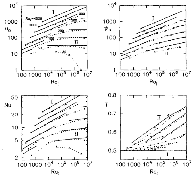
FIG. 6. The numerical 14 (solid boxes) and corresponding theoretical (solid lines) dependences of u_0 , Nu , \psi_m , and T as functions of Ra_i \approx Ra_i are shown for non-Newtonian ( n=3 ) temperature-dependent viscosity convection. The Rayleigh number Ra_0 is fixed along each curve ( Ra_0 = 50, 100, 250, 500, 1000, 2000 ). Two convective regimes are: I—the small viscosity contrast regime and II—the transitional regime. The numerical data for Ra_0 = 32 (triangles) do not obey the formulas suggested for these two regimes and, probably, indicate a transition to the third regime. This is shown in Fig. 7.
