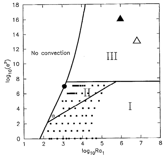
FIG. 8. The three convective regimes are very approximately shown in Ra_1 - \exp(p) axes for non-Newtonian viscosity convection ( n=3 ). The numerical data 13 are marked with solid boxes. The point where the layer was convectively stable is marked with an open box. The formal locations of the Earth's mantle with the temperature T_i=1773 K and with the rheology of "wet" (an open triangle) and "dry" (a solid triangle) olivine 34 with n \approx 3-3.5 are indicated.
