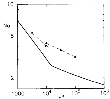
FIG. 3. The data showing the transition from whole-layer to stagnant lid convection (open and solid triangles respectively) 16 are plotted in the coordinates used by Ogawa et al. 16 Nusselt number versus the viscosity contrast \exp(p) . The Rayleigh number Ra_1 = 3.2 \times 10^6 based on the viscosity of the bottom is fixed. The corresponding theoretical curve is shown with a solid line.
