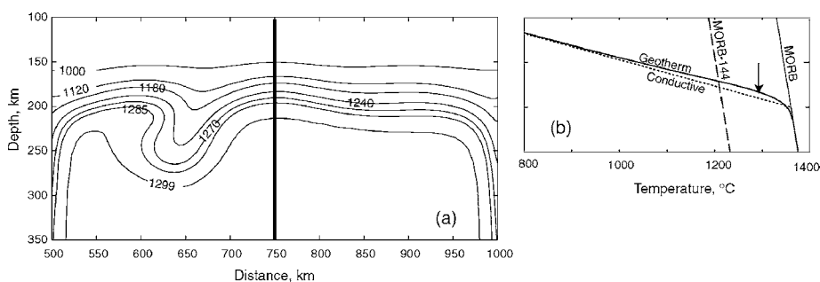
Figure 5 Potential temperature contours show convection beneath a stagnant lid (a). The dark line shows the position of the geotherm sampled in panel (b). From theory in Equation 10, the rheological boundary contrast should be 144 K. This quantity would be obtained from the laterally averaged temperature. The computed geotherm, however, has a break in slope at only \sim 70 K (arrow). From model in figure 1 of Sleep (2003b).
