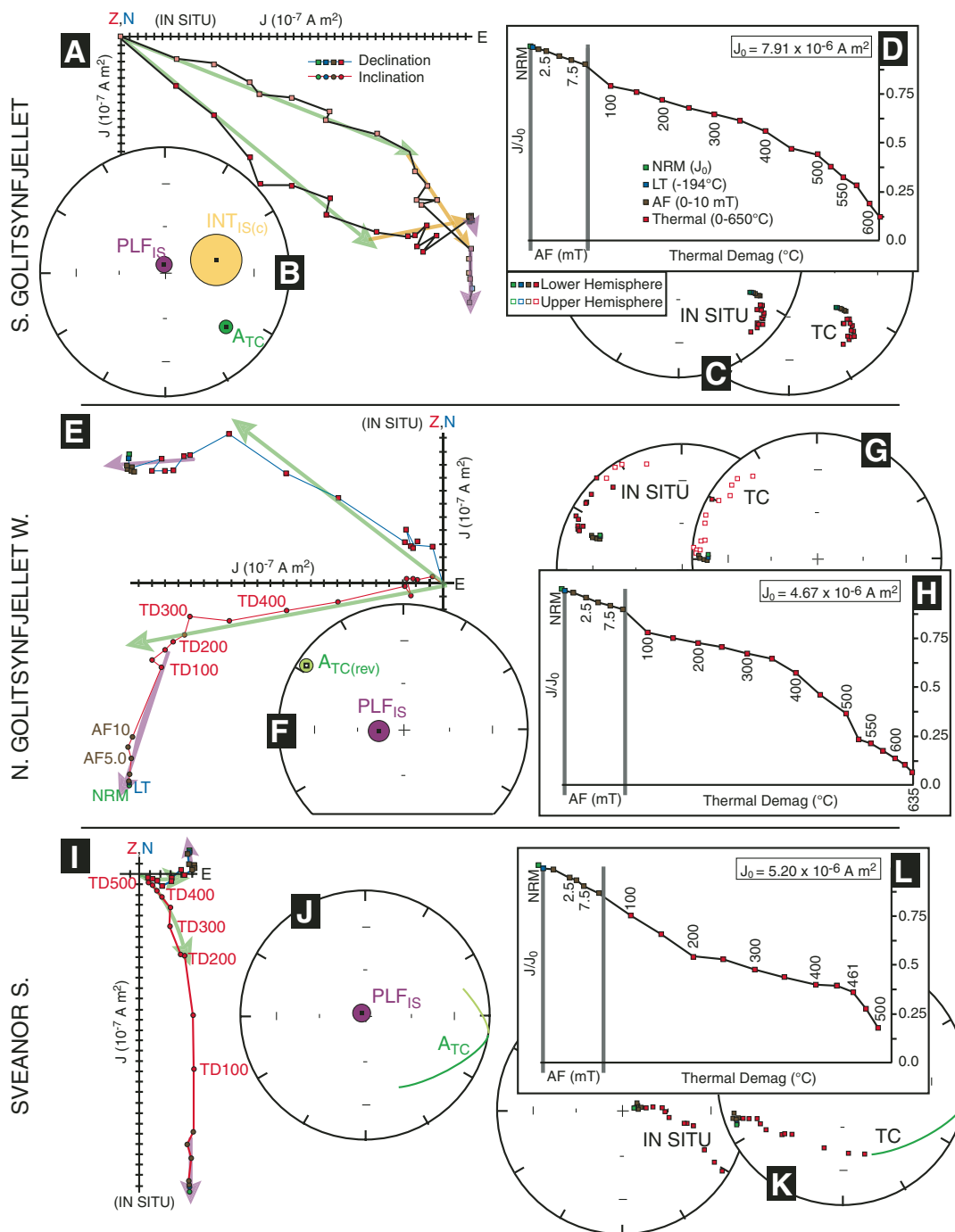
Figure 4. Representative vector component diagrams (Zijderveld, 1967) (A, E, and I), least-squares fits (B, F, and J), equal-area projections (C, G, and K) and magnetic intensity ( J/J_0 ) plots (D, H, and L) showing demagnetization behavior for the Upper Grusdievbreen Formation (uGfm). In the Zijderveld plots (always in situ coordinates), the primary, high-temperature component that decays to the origin is traced with a green arrow, intermediate directions, when present, are traced with a yellow arrow, and the present local field (PLF) overprint is traced with a purple arrow. When thermal unblocking spectra are arcuate, rather than linear, a great circle is fit to the data instead of a line (I–K). Least-squares fits of these components, with error ovals representing circular maximum angular deviation (MAD) angles from the principal component analysis (plotted using the routines of Cogné [2003] and Jones and Tetreault [2004]), are summarized in an adjacent equal-area projection (B, F, and J), and are labeled A_{TC} , INT_{IS(c)} , and PLF_{IS} , respectively, where TC refers to tilt-corrected and IS refers to in situ coordinates. In all plots, green-filled shapes are natural remanent magnetization (NRM) directions, blue-filled shapes are the low-temperature step, brown-filled shapes reflect alternating field (AF) demagnetization steps, and red-filled shapes reflect thermal demagnetization. In the Zijderveld plots (A, E, and I), squares/circles represent declination/inclination, while in the equal-area nets (C, G, and K), color-filled/color-rimmed squares represent lower/upper-hemisphere directions.
