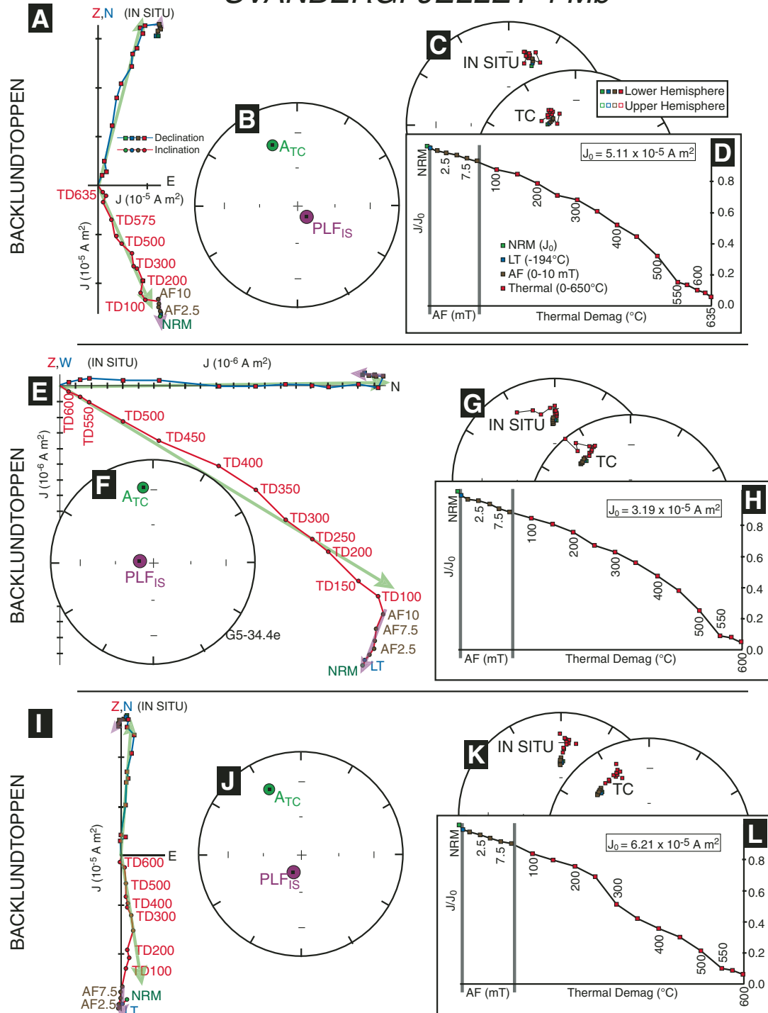
Figure 3. Representative vector component diagrams (Zijderveld, 1967) (A, E, and I), least-squares fits (B, F, and J), equal-area projections (C, G, and K), and magnetic intensity ( J/J_0 ) plots (D, H, and L) showing demagnetization behavior for the Svanbergfjellet 4 Member (S4mb). In the Zijderveld plots (always in situ coordinates), the primary, high-temperature component that decays to the origin is traced with a green arrow, and the present local field (PLF) overprint is traced with a purple arrow. Least-squares fits of these components, with error ovals representing circular maximum angular deviation (MAD) angles from the principal component analysis (plotted using the routines of Cogné [2003]), are summarized in an adjacent equal-area projection (B, F, and J), and are labeled A TC and PLF IS , respectively, where TC refers to tilt-corrected and IS refers to in situ coordinates. In all plots, green-filled shapes are natural remanent magnetization (NRM) directions, blue-filled shapes are the low-temperature step, brown-filled shapes reflect alternating field (AF) demagnetization steps, and red-filled shapes reflect thermal demagnetization. In the Zijderveld plots (A, E, and I), squares/circles represent declination/inclination, while in the equal-area nets (C, G, and K), color-filled/color-rimmed squares represent lower/upper-hemisphere directions.
