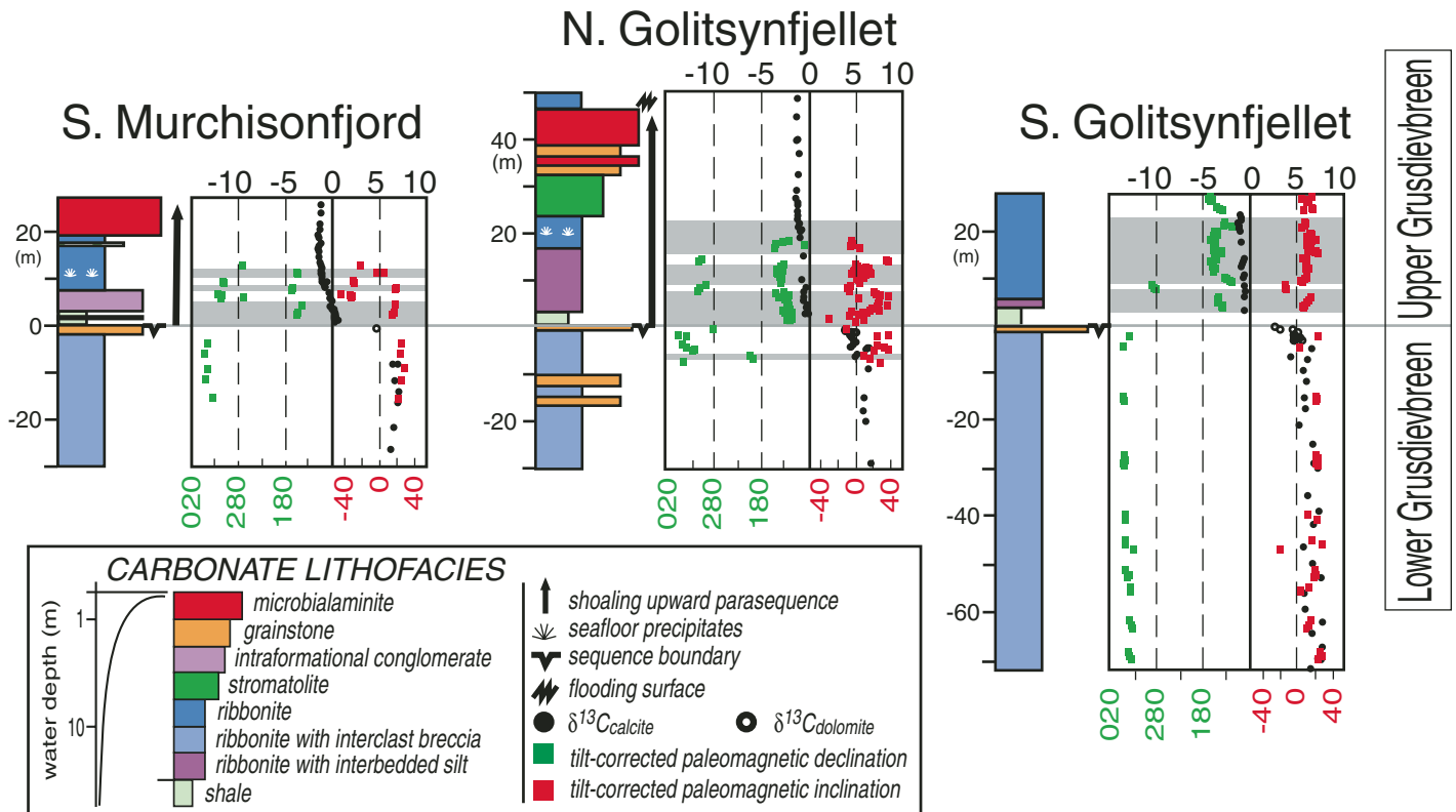
Figure 7. Paleomagnetic and carbon-isotope stratigraphy across the G1 sequence boundary. Carbon isotope data for calcite/dolomite are plotted with solid/open black circles, while tilt-corrected paleomagnetic declination and inclination are plotted with solid green and red squares, respectively. White and gray areas correspond to opposite magnetic polarities. Stratigraphic height is set to 0 meters at the G1 sequence boundary. Carbonate lithofacies are color coded, and wider boxes reflect depositional environments in shallower water. Seafloor precipitates are thought to be calcite pseudomorphs after aragonite.
