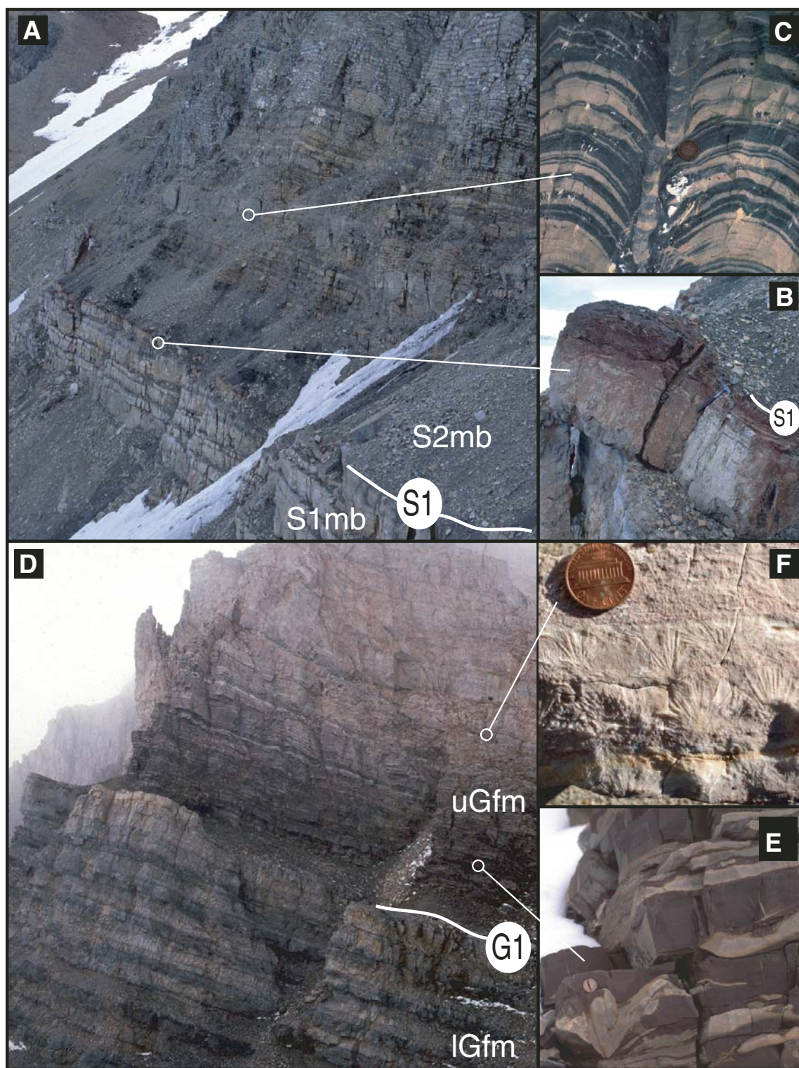
Figure 2. Field photographs of the Grusdievbreen and Svanbergfjellet Formations. (A) S1 sequence boundary (white line) separating Svanbergfjellet 1 (S1mb) and Svanbergfjellet 2 (S2mb) members at Svanbergfjellet (Fig. 1C). Despite brecciation, silicification, and ferruginization of the sequence boundary (B), there is no evidence of erosional relief on the outcrop scale (in B, hammer is 33 cm long). (C) Minjaria sp. stromatolites form a distinctive biostrome 10–15 m above the S1 boundary throughout northeast Svalbard (Knoll and Swett, 1990). (D) G1 sequence boundary (white line) separating the Upper (uGfm) and Lower (lGfm) Members of the Grusdievbreen Formation at North Golitsynfjellet (Fig. 1C). Note the ~2 m of karstic relief on the dolomitized (beige) G1 contact and the sharp change in parasequence lithology above the boundary. A green silt fills in the erosional relief on G1, and is overlain by edgewise limestone breccias (E) and aragonite pseudomorphs (“crystal fans”) that form a continuous seafloor cement (F). Pennies in C, E, and F are 1.9 cm in diameter.
