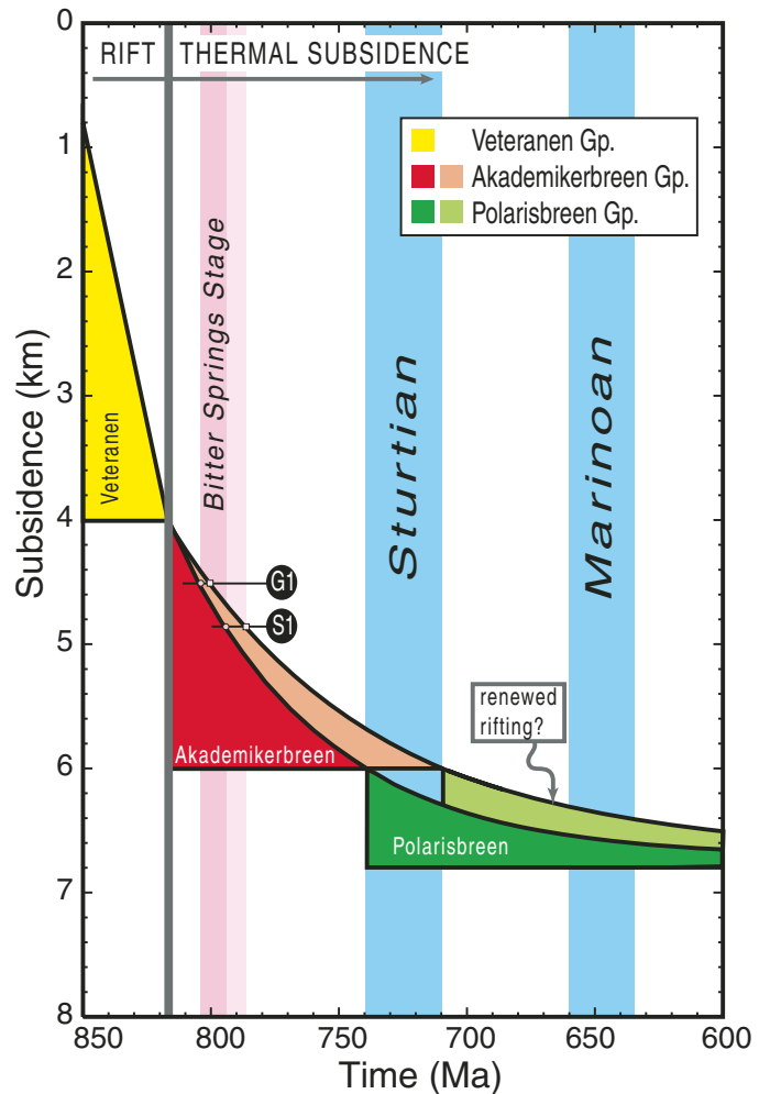
Figure 10. Age model for the Hecla Hoek strata of East Svalbard. The black curves show rifting (Veteranen Group) and thermal subsidence (Akademikerbreen Group) of an originally 35-km-thick continental crust and 100-km-thick lithosphere. The dark/light colored triangular areas beneath the solid curves depict the age distribution of the continuum of stratigraphic levels assuming onset of Sturtian glaciation at ca. 740 and ca. 710 Ma, respectively. The Akademikerbreen Group was deposited in ~90 m.y., and the entire Bitter Springs Stage lasted ~12 m.y. Discussion of the Polarisbreen Group is beyond the scope of this paper; however, it is worth noting that the post-Sturtian subsidence curve is more complicated than shown and should incorporate both (1) compaction of Polarisbreen shales, and (2) the possibility of renewed rifting (Herrington and Fairchild, 1989).
