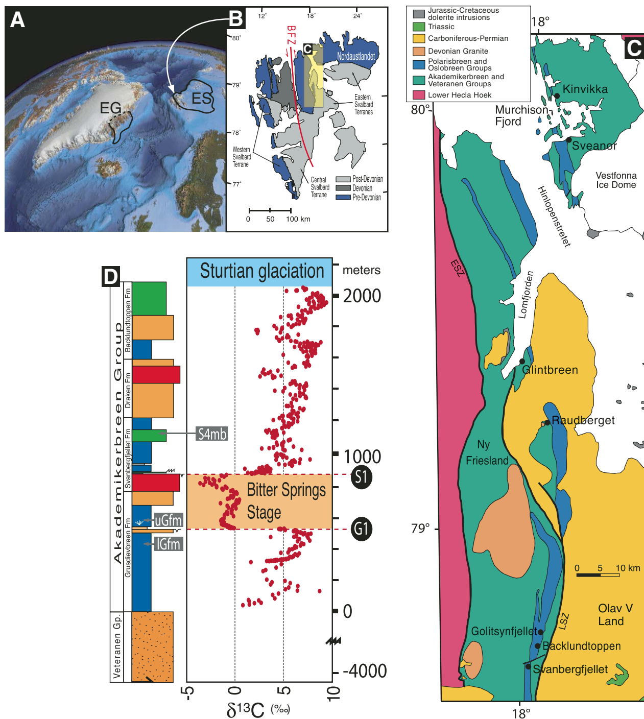
Figure 1. (A) The Svalbard archipelago is located on the northwest edge of the Barents Shelf and is composed of (B) three distinct tectonic terranes (western, central, and eastern), which were juxtaposed via sinistral transpression along the Billefjorden (BFZ) and other north-south fault zones during Silurian-Devonian times. East Greenland (EG) and East Svalbard (ES, also known as Barentsia) are thought to have been part of a contiguous Neoproterozoic basin (EGES) in Eastern Laurentia (A). The semitransparent yellow box in B marks the coverage of the generalized geologic map in C, after Harland (1997), which shows the locations of our measured stratigraphic sections through the Akademikerbreen Group that are mentioned in the text. In C, note the positions of (1) the Cretaceous sills west of Glintbreen, (2) the small Devonian intrusion west of Raudberget, and (3) the Lomfjorden shear zone (LSZ) east of Backlundtoppen, and (4) the Eoluseltta shear zone (ESZ) separating Lower Hecla Hoek metamorphic rocks to the west from Neoproterozoic rocks to the east. (D) A composite stratigraphic section (see Fig. 7 for a key to the carbonate lithostratigraphy) of the Akademikerbreen Group showing the \delta^{13}\text{C} record (Halverson et al., 2005, 2006), along with the locations of the G1 and S1 sequence boundaries sandwiching the Bitter Springs isotope stage (Halverson et al., 2005). Also shown are the stratigraphic position of the Lower Grusdievbreen (IGfm), Upper Grusdievbreen (uGfm), and Svanbergfjellet (S4mb) paleomagnetic sampling horizons.
