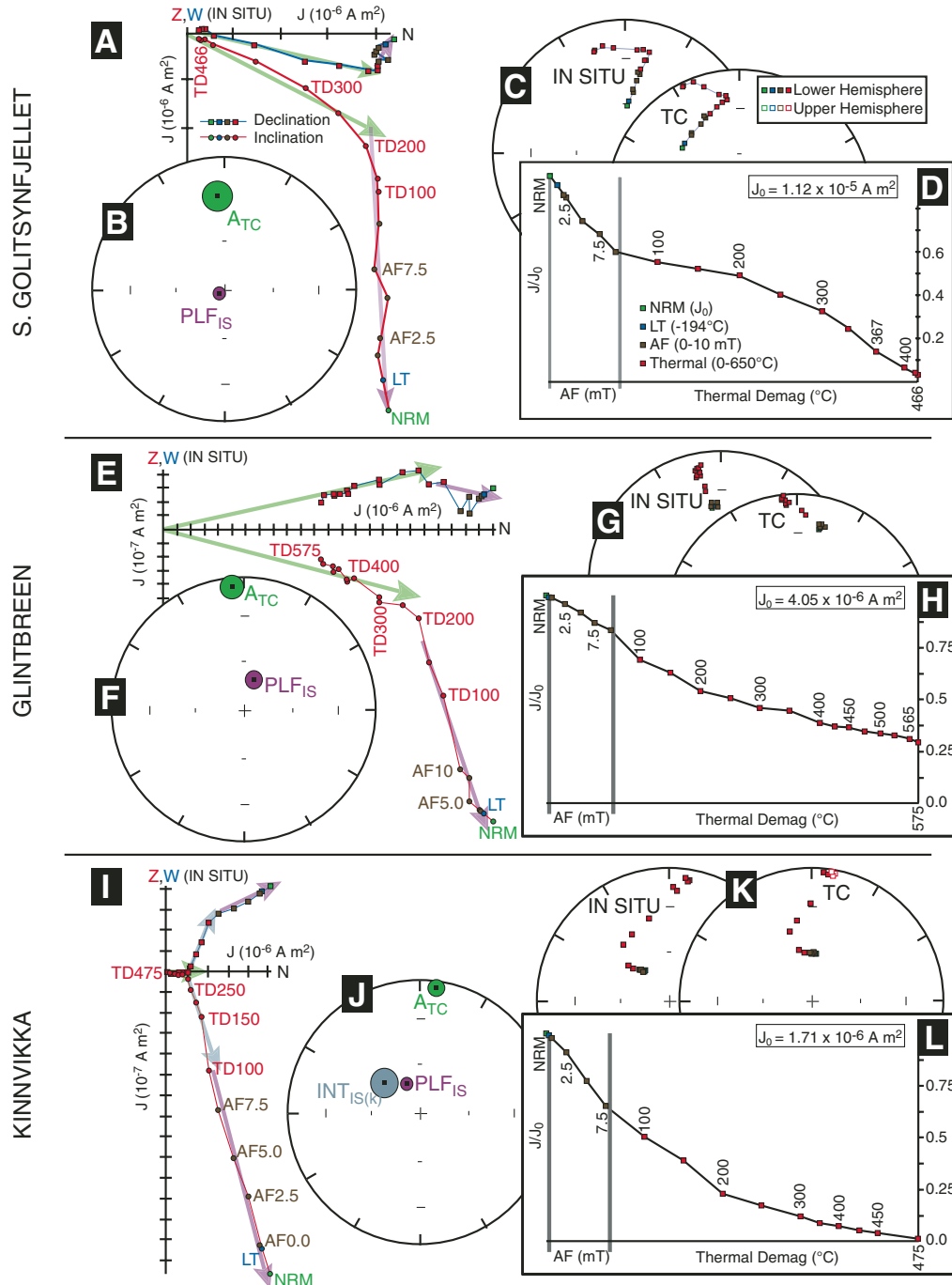
Figure 5. Representative vector component diagrams (Zijderveld, 1967) (A, E, and I), least-squares fits (B, F, and J), equal-area projections (C, G, and K) and magnetic intensity ( J/J_0 ) plots (D, H, and L) showing demagnetization behavior for the Lower Grusdievbreen Formation (IGfm). In the Zijderveld plots (always in situ coordinates), the primary, high-temperature component that decays to the origin is traced with a green arrow, intermediate directions, when present, are traced with a gray arrow, and the present local field (PLF) overprint is traced with a purple arrow. Least-squares fits of these components, with error ovals representing circular maximum angular deviation (MAD) angles from the principal component analysis (plotted using the routines of Cogné [2003]), are summarized in an adjacent equal-area projection (B, F, and J), and are labeled A_{TC} , INT_{IS(k)} , and PLF_{IS} , respectively, where TC refers to tilt-corrected and IS refers to in situ coordinates. In all plots, green-filled shapes are natural remanent magnetization (NRM) directions, blue-filled shapes are the low-temperature step, brown-filled shapes reflect alternating field (AF) demagnetization steps, and red-filled shapes reflect thermal demagnetization. In the Zijderveld plots (A, E, and I), squares/circles represent declination/inclination, while in the equal-area nets (C, G, and K), color-filled/color-rimmed squares represent lower/upper-hemisphere directions.
