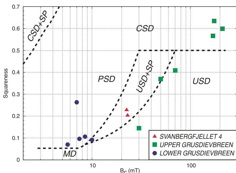
Figure 9. Summary plot of squareness ( M_r/M_s ) versus coercive field ( B_c ) for Svanbergfjellet (S4mb), Upper Grusdievbreen (uGfm), and Lower Grusdievbreen (IGfm) samples. Dashed black lines delineate approximate boundaries for magnetite size fractions, where CSD is hypothetical cubic single domain, SP is superparamagnetic, USD is uniaxial single domain, PSD is pseudo-single domain, and MD is multidomain (Tauxe et al., 2002).
