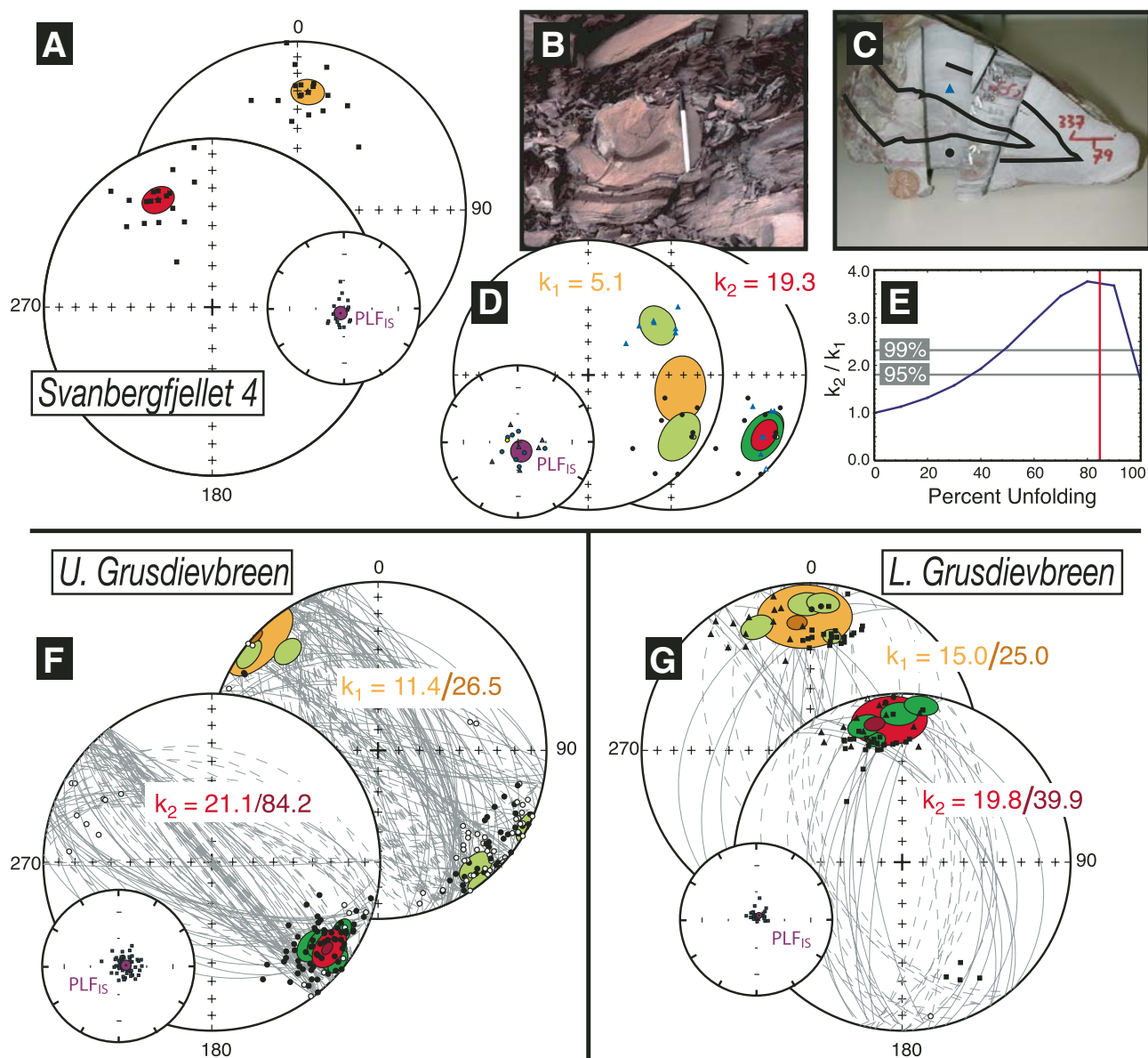
Figure 6. Tests for the presence of prefoling or synfoling magnetization. Equal-area nets show in situ (orange) and tilt-corrected (red) Fisher distributions of the characteristic remanent magnetization (ChRM) direction and in situ distribution of the present-local field (PLF) overprint (purple) for the Lower Grusdievbreen (IGfm) (G), Upper Grusdievbreen (uGfm) (F), and Svanbergfjellet (S4mb) (A). Filled/open circles are lower/upper-hemisphere least-squares line fits to demagnetization curves. Gray arcs are great circle fits to demagnetization curves with overlapping magnetic components. Where multiple stratigraphic sections are present, as in (F) and (G), individual section-mean Fisher statistics are plotted as light green (in situ) and dark green (tilt-corrected) ellipses, while the averages of section-mean directions are plotted as dark orange (in situ) and dark red (tilt-corrected) ellipses. Values k_1 and k_2 are in situ and tilt-corrected Fisher (Fisher, 1953) concentration parameters measuring the dispersion in individual paleomagnetic data (light orange and light red) and site-mean paleomagnetic data (dark orange and dark red). S4mb contains numerous disturbed beds of pink limestone and red marl with detached synsedimentary folds (B) and erosional truncations (left of the pen cap in B). Paleomagnetic directions from the upper limb (blue triangles) and lower limb (black circles) of the fold pictured in C are plotted on the equal-area net in D. The PLF overprint direction fails the fold test, while the primary magnetic component passes the synsedimentary fold test at the 99% confidence level (E). (E) Shows that k_2/k_1 is maximized at 86% unfolding and that the S4mb ChRM was likely acquired prior to, or at the onset of slump folding, and thus dates from the time of sedimentation. (Note: the demagnetization behavior of the ChRM from A and D is identical, and the two directions are considered to reflect the same paleomagnetic component. The difference in absolute direction of the ChRM in D with respect to the ChRM in A is just another reflection of the observation that the ChRM was acquired prior to disruption and folding.) Both the uGfm (F) and IGfm (G) directions were derived from multiple stratigraphic sections separated by >100 km. Although paleomagnetic directions are subparallel to the NNW-trending Caledonian fold axes, k_2/k_1 is maximized at 100% unfolding, and both uGfm and IGfm pass the McElhinny (1964) fold test at greater than the 92% confidence level.
