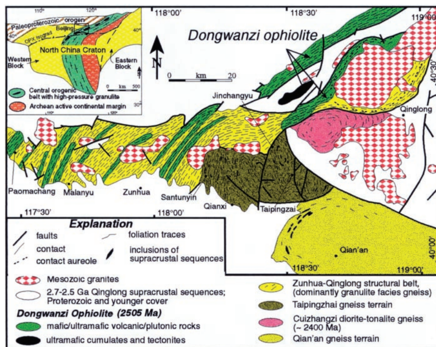
Fig. 1. Map of part of the eastern Hebei Province, North China craton, showing the location and tectonic setting of the Dongwanzi ophiolite. There are abundant similar belts of amphibolite-granulite-grade metabasites in the Zunhua structural belt. The inset shows major tectonic divisions of the North China craton, into the western and eastern blocks, Central orogenic belt, and Paleoproterozoic orogenic belt [after (9)].
