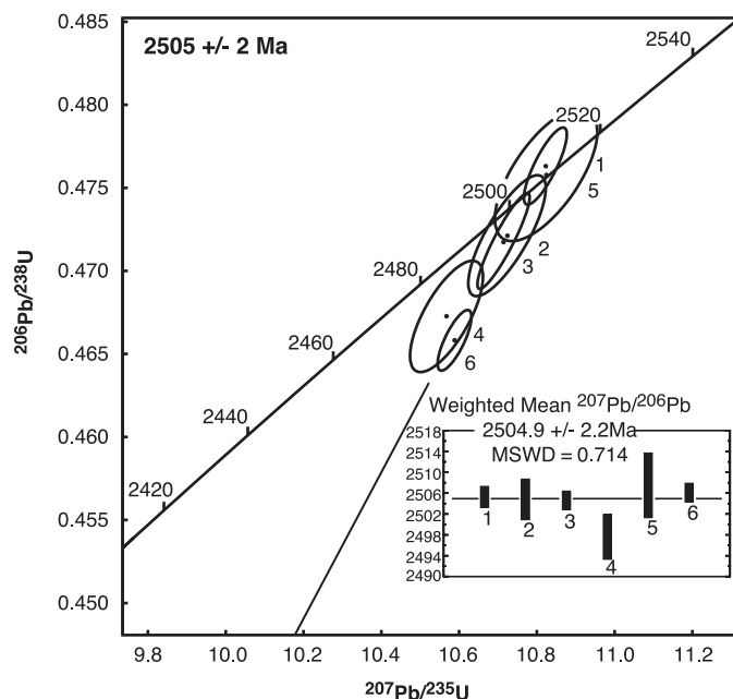
Fig. 4. Concordia plot of zircons from the Dongwanzi ophiolite gabbros, showing an age of 2505 \pm 2.2 Ma for the ophiolite. MSWD, mean square weighted deviation.
