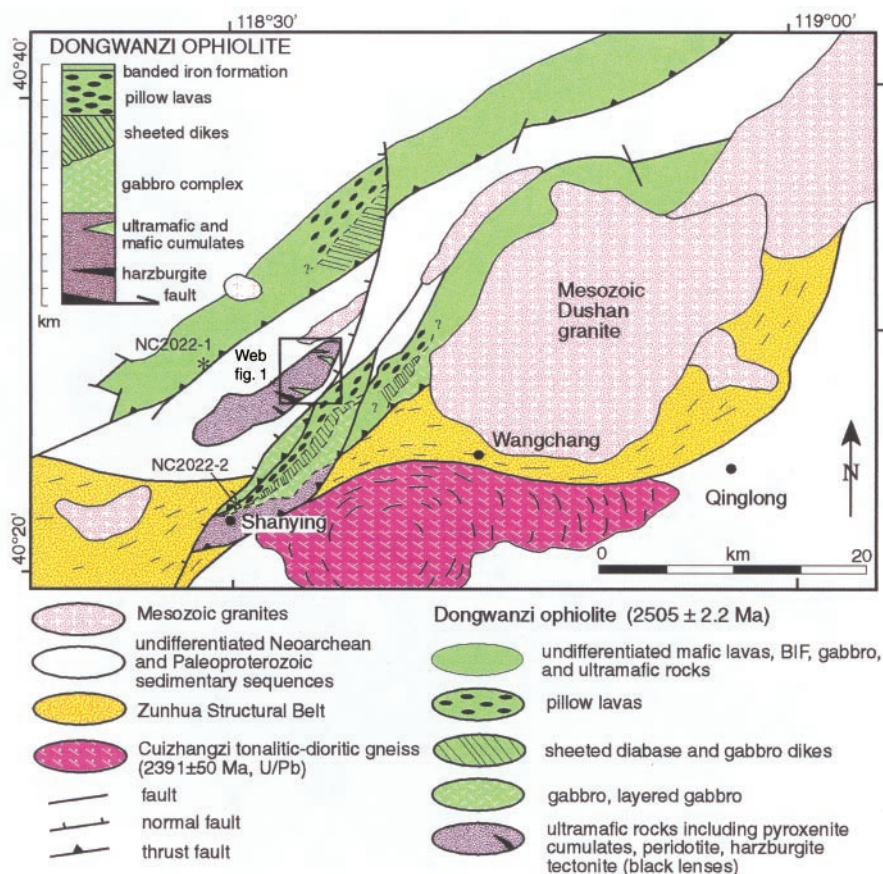
Fig. 2. Reconnaissance map of the Dongwanzi ophiolite, showing belts of pillow lavas, sheeted dikes, gabbro complex, cumulate ultramafic rocks, and harzburgite tectonite. The column to the top left shows the thickness of units on the basis of map patterns. The Dongwanzi ophiolite is intruded by the (deformed) ~2.4-Ga Cuizhangzi gneiss (12). We have obtained a U-Pb zircon age of 2505 ± 2.2 Ma for gabbro from the Dongwanzi ophiolite (sample locations shown by an asterisk). Sites NC2022-1 and NC2022-2 show locations of geochronology samples. Question marks indicate approximate boundaries of mapping where internal units of ophiolite have been delineated.
