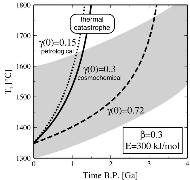
Figure 2. Thermal evolution modeling with conventional heat flux scaling of equation (11). The activation energy is set to 300 kJ/mol. Three present-day Urey ratios are used: 0.15 (petrological, dotted), 0.3 (cosmochemical, solid), and 0.72 (superchondritic, dashed). Gray shading denotes the range of potential temperatures recorded in MORB-like suites including greenstone belts and ophiolite suites Figure 5 [Abbott et al. , 1994, their Figure 5].
