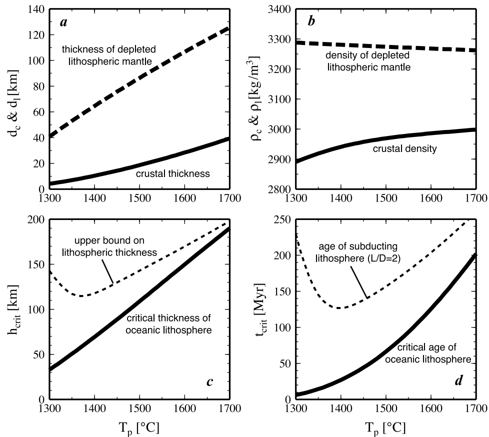
Figure 9. Compositional buoyancy of oceanic lithosphere and its subductability as a function of mantle potential temperature. (a) Thickness of oceanic crust (solid) and depleted mantle (dashed). (b) Density of oceanic crust (solid) and depleted mantle (dashed). Crustal density increases with potential temperature because higher degree of melting increases the olivine content of resulting crust. (c) Critical thickness for net negative buoyancy (solid). Upper limit for the thickness of oceanic lithosphere when dehydration stiffening is present (Figure 5) is also shown as dashed. (d) Critical plate age for subduction (solid). Dashed curve denotes the age of subducting plate assumed in the heat-flow parameterization for plate-tectonic convection.
