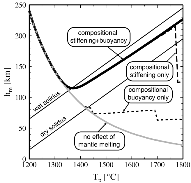
Figure 5. Maximum plate thickness as a function of mantle potential temperature. As in Figure 4, reference viscosity is 10^{19} Pa s at 1350^{\circ}\text{C} , and activation energy for temperature-dependent viscosity is set to 300 kJ/mol. Gray curve corresponds to this purely temperature-dependent viscosity. Dotted line shows the effect of added compositional buoyancy, dashed line shows the effect of added compositional stiffening, and solid line shows the effects of adding both. For comparison, dry and wet solidi are also shown. Plate thickness for T_p > 1350^{\circ}\text{C} roughly follows the wet-to-dry transition.
