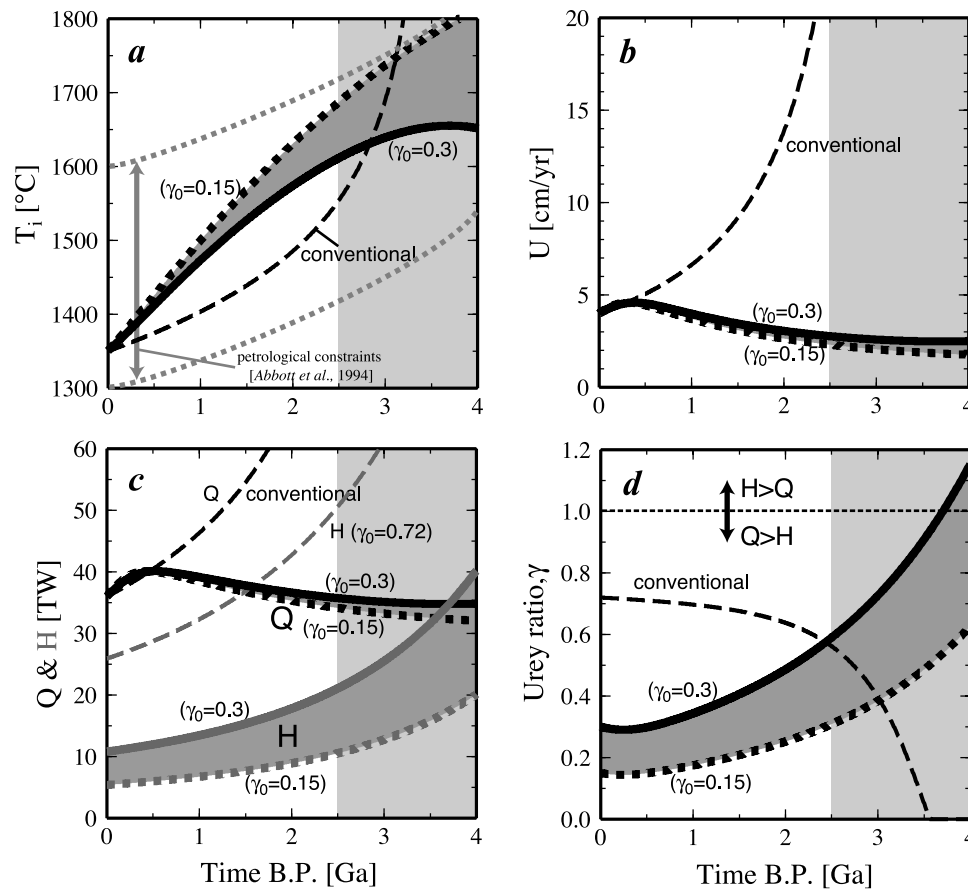
Figure 7. Thermal evolution modeling incorporating the energetics of plate-tectonic convection, with the Urey ratio of 0.15–0.3. For comparison, results from the conventional model with the Urey ratio of 0.72 (Figure 2) are also shown as dashed curve. (a) Mantle internal temperature. (b) Plate velocity. (c) Surface heat flux Q and internal heating H . (d) Urey ratio. Gray shading for > 2.5 Ga indicates large uncertainty involved in predicted thermal history, i.e., heat flux scaling to be used may be considerably different in this time range. In (a), the range of potential temperatures recorded in MORB-like suites [Abbott et al. , 1994] is also shown as dotted lines.
