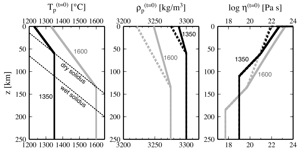
Figure 4. Zero-age oceanic mantle profiles for two potential temperatures of unmelted mantle: 1350°C (solid) and 1600°C (gray). (left) Potential temperature. Dry solidus is based on Takahashi and Kushiro [1983], and wet solidus is placed 50 km below dry solidus. A constant melting rate (after crossing dry solidus) of 10%/GPa is assumed, and H_f/c_p is set to 600 K. (middle) Potential density. Dashed lines denote the case of melt depletion effect only. The effect of cooling due to the latent heat of fusion is incorporated in solid lines. (right) Viscosity. Reference viscosity (for oceanic upper mantle) is 10^{19} Pa s at 1350°C [ Hager, 1991; Karato and Wu, 1993; Hirth and Kohlstedt, 1996; Korenaga and Jordan, 2002b ], and activation energy for temperature-dependent viscosity is set to 300 kJ/mol. Dehydration stiffening is modeled as 100-fold viscosity increase during the wet-to-dry transition, followed by 3-fold increase per every additional 10% of melting. Dashed lines show the effect of dehydration whereas solid lines incorporate cooling upon melting.
