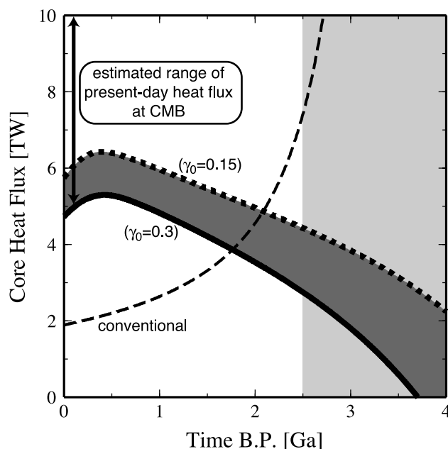
Figure 11. The first-order thermal history of the core. Legend is the same as in Figure 7. Core heat flux is calculated as \sim 19\% of the whole-Earth secular cooling [Stacey, 1981].
