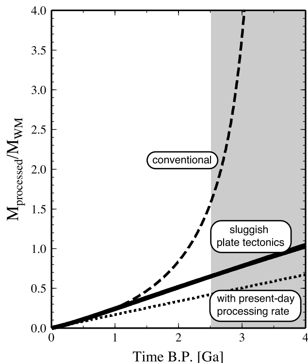
Figure 12. Efficiency of mantle mixing in terms of processed mantle mass normalized by the mass of the whole mantle. Because of the trade-off between plate velocity and the initial depth of mantle melting, the difference in the assumed Urey ratio (i.e., 0.15 or 0.3) results in negligible difference in the processing rate (solid curves). Dashed curve denotes the prediction based on the convection model with the Urey ratio of 0.72. A hypothetical case with the constant processing rate of the present-day value is also shown as dotted. Sluggish plate tectonics is characterized by low processing rates similar to this extreme case.
