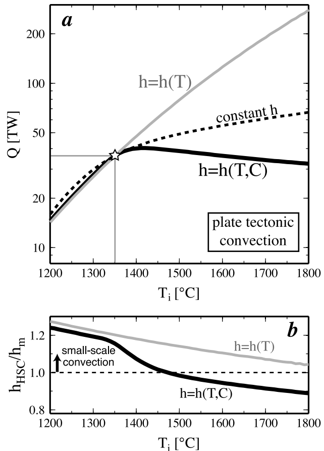
Figure 6. (a) Heat flux parameterization for plate-tectonic convection (equation (19)). Dotted curve is for the case of constant plate thickness of 100 km. The case of purely temperature-dependent viscosity is denoted by gray lines, and that of compositional stiffening and buoyancy is by solid lines. (b) The role of small-scale convection in regulating maximum plate thickness ( h_m ) is shown by comparing with hypothetical thickness by half-space cooling only ( h_{\text{HSC}} ). See text for discussion.
