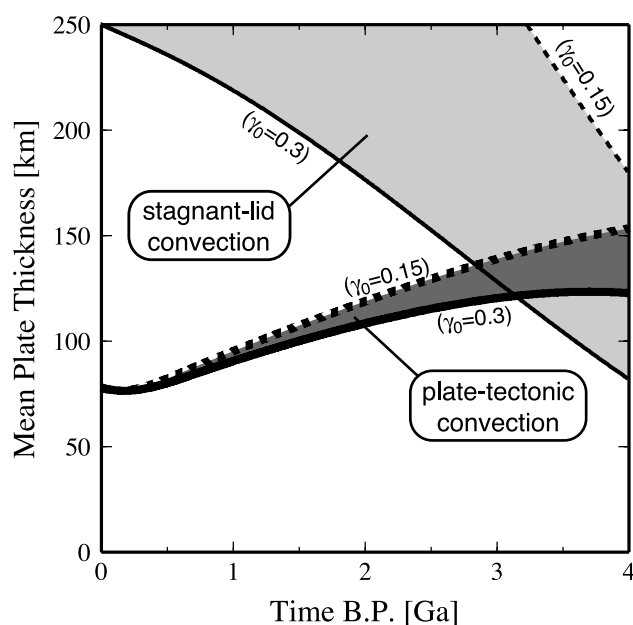
Figure 10. Mean plate thickness for plate-tectonic convection and stagnant-lid convection. Stagnant-lid convection is assumed to be in equilibrium with internal heat production. Thermal conductivity k is set to 4 \text{ W m}^{-1} \text{ K}^{-1} in equation (38).
