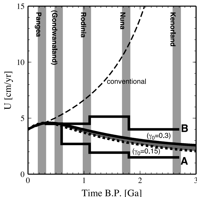
Figure 8. Comparison of predicted plate velocity with the geological estimate based on the history of supercontinents. Legend for model prediction is the same as in Figure 7b. Gray bars denote the periods of supercontinent assemblies based on Hoffman [1997]. Case A is a geological estimate based on five “supercontinents”: Pangea, Gondwanaland, Rodinia, Nuna, and Kenorland. Plate velocity is calculated as the reciprocal of the recurrence interval, and is scaled with 4.5 \text{ cm yr}^{-1} for the Pangea-Gondwanaland interval to line up with the model prediction at 0.3 Ga for comparison. Case B is based on four supercontinents, Pangea, Rodinia, Nuna, and Kenorland. The same velocity scaling is applied with the Pangea-Rodinia interval.
