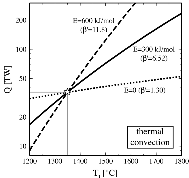
Figure 1. “Conventional” heat flux parameterization based on Nu-Ra scaling and single mantle rheology (equation (11)). Three cases are shown: (1) E = 0 (dotted, a' = 3.07 \times 10^{-3} , \beta' = 1.30 ), (2) E = 300 kJ/mol (solid, a' = 1.35 \times 10^{-19} , \beta' = 6.52 ), and (3) E = 600 kJ/mol (dashed, a' = 5.95 \times 10^{-36} , \beta' = 11.8 ). Star denotes the present-day mantle condition, to which the scaling law is calibrated.
