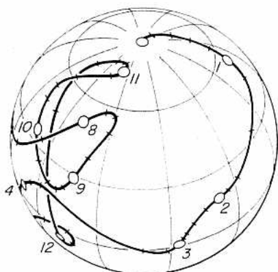
Fig. 3. A simulated curve of polar wandering. The meridians and the circles of latitude on the sphere are both drawn 30^\circ apart. The markers along the path denote 'time' t = 0.2, 0.4, 0.6 , etc.
