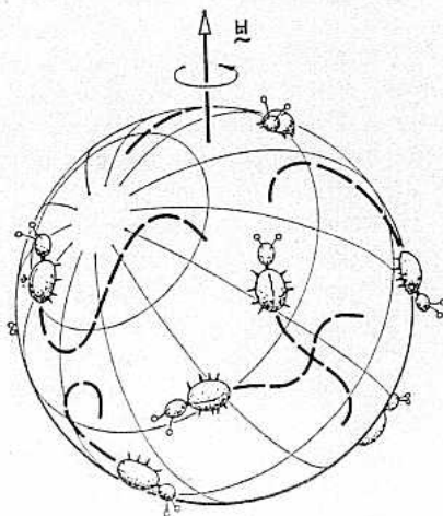
Fig. 1. A quasi-rigid body.
