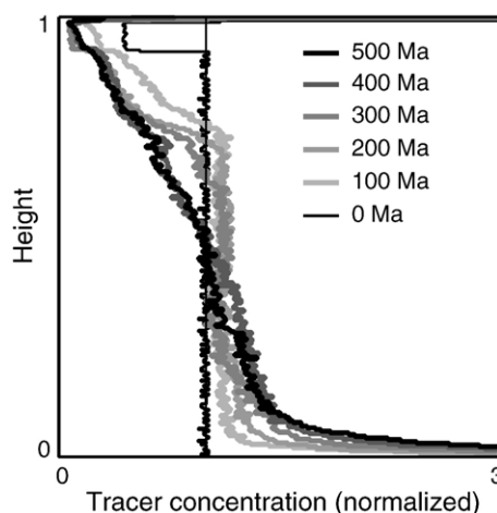
Fig. 2. Vertical profiles of horizontally averaged tracer concentration at various times in the model shown in Fig. 1. Tracer concentration is normalised to the average concentration in the model, revealing a rapid depletion of the upper mantle, a slight enrichment of the lower mantle and a strongly enriched thin layer at the base. The concentration in the basal layer reaches (and is limited to) about 10, corresponding to pure mafic material.
