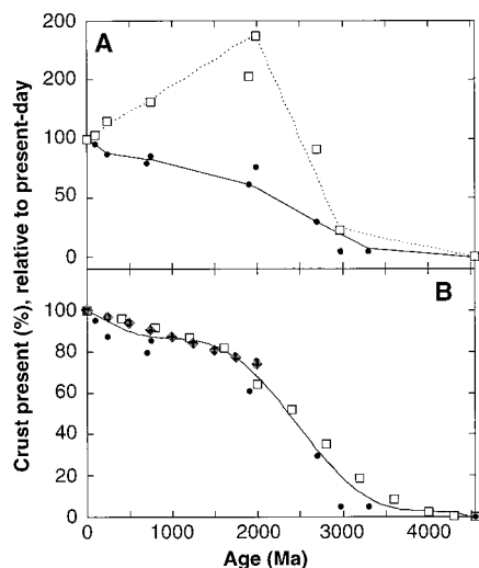
Fig. 2. Curves for crust volume versus age. (A) Comparison of crust volumes estimated through the Nb/Th ratio (filled circles, connected by solid line) and through the Nb/U ratio (open squares, connected by dotted line). Estimation is based on the assumption that the chondritic values represent 0% crust and that present-day MORB average represents 100% of present continental crust volume. Note that the Nb/U-based estimate predicts the former existence of a substantially more voluminous continental crust. (B) Comparison of crust volumes estimated from geophysical data by Reymer and Schubert (15) (solid diamonds), transport-forward modeling by Kramers and Tolstikhin (9) (open squares), and the Nb/Th evolution of the depleted mantle in (A) (solid circles). Solid line represents composite parameterization for the crust volume versus age (eight data points from Reymer and Schubert, 12 data points from Kramers and Tolstikhin, and all 10 Nb/Th data points). Relative to the present-day volume or mass of continental crust, the percent volume or mass of continental crust ( y ) present at any given age ( t , in megannum) can be expressed as a seven-order polynomial: y = 100 - 1.5742 \times 10^{-2} \times t - 4.2617 \times 10^{-5} \times t^2 + 9.9543 \times 10^{-8} \times t^3 - 7.663 \times 10^{-11} \times t^4 + 2.5738 \times 10^{-14} \times t^5 - 3.9626 \times 10^{-18} \times t^6 + 2.3005 \times 10^{-22} \times t^7 with r^2 = 0.984 .
