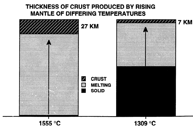
Figure 6. Illustration of melting column model. Hotter mantle begins to melt at a greater depth and produces thicker oceanic crust. Colder mantle begins to melt at lower depths and produces thinner oceanic crust.
