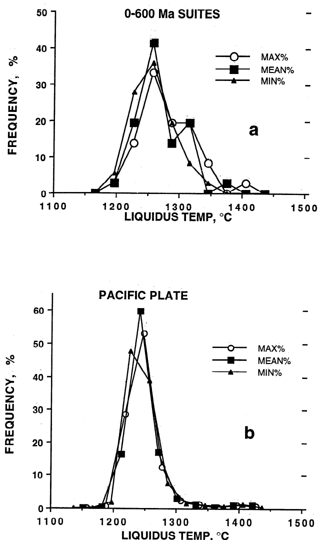
Figure 8. Three percentage areas are shown: MIN, MEAN, and MAX. (a) Distribution of liquidus temperatures derived from the most primitive rock in each of 36 Phanerozoic ophiolite suites compiled for this study. The minimum, mean and maximum histograms were calculated using the error bars for the temperature values in Table 1. (b) Distribution of liquidus temperatures calculated from the residual depth anomalies in the modern Pacific plate. The minimum, mean and maximum histograms are the result of using different bin midpoints for the data.
