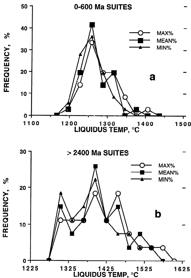
Figure 4. (a) Graph of the liquidus temperatures obtained for the Phanerozoic (0-600 Ma). (b) Graph of the liquidus temperatures obtained for the Archean (2400 Ma to 3800 Ma). Data for both figures obtained using the methods outlined in text. Three percentage areas are shown: MIN, MEAN, and MAX. The shapes of the two distributions are very similar, i.e., both are unimodal, skewed distributions. This indicates that the relative proportion of hotspot volcanism has not changed much over geologic time.
