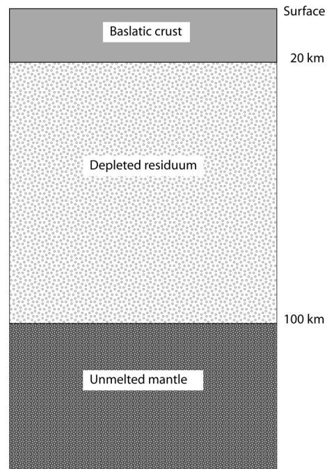
Figure 6 Section through oceanic lithosphere where upwelling mantle starts melting at 100 km depth. This lithosphere is difficult to subduct. Both the crust and depleted residuum are buoyant relative to the underlying mantle. Unlike basaltic mush, the depleted residuum is quite viscous and does not internally convect.
