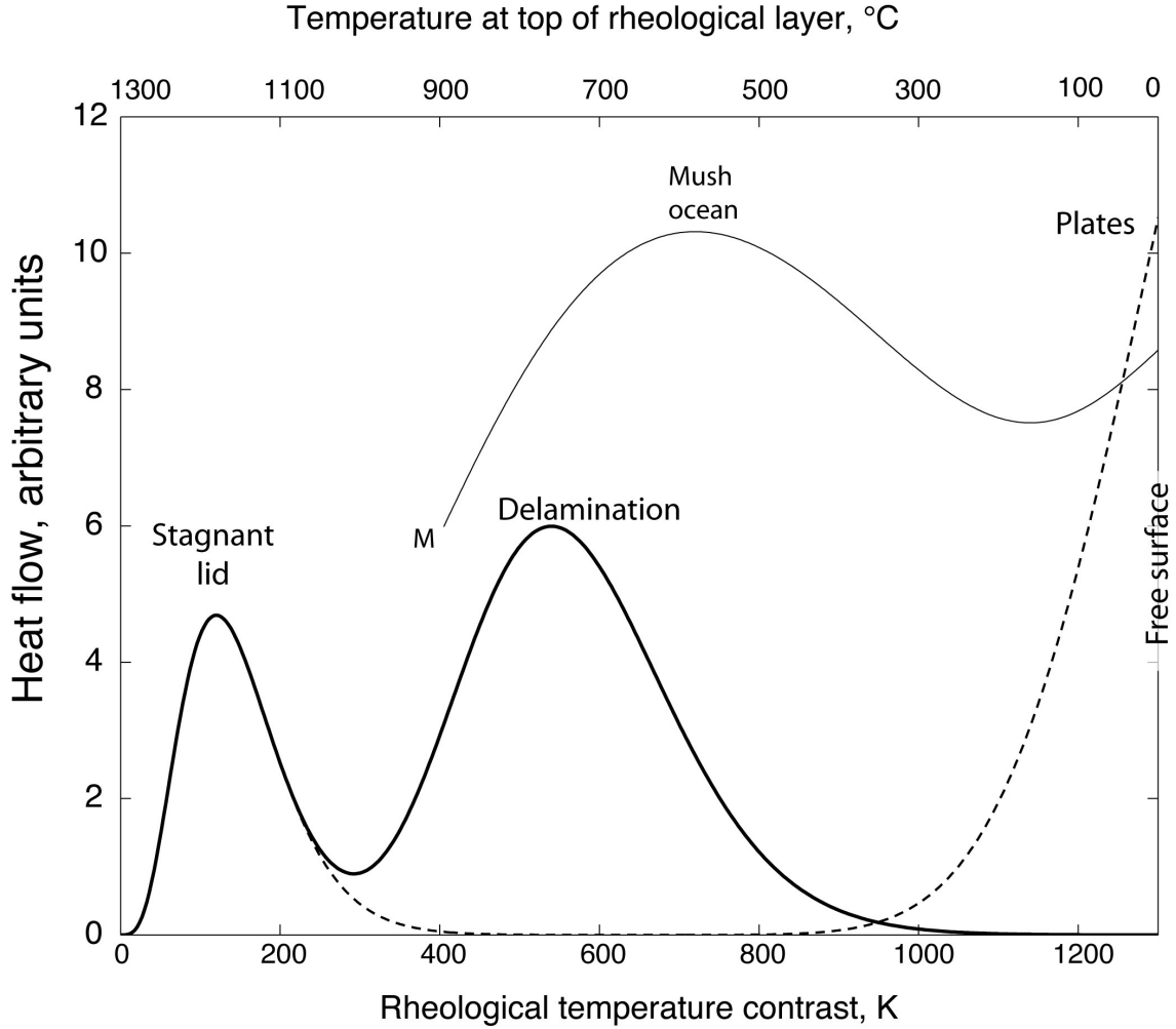
Figure 5 The heat flow in arbitrary units from (19). I have adjusted the constant a in each model so that the amplitude of the peaks is comparable for schematic plotting convenience. The second peak of the solid curve corresponds to delamination of the lithosphere, n = 8 . The dashed curve represents plate tectonics. The computed heat flow is still increasing when the rheological temperature contrast is equal to its maximum possible value, the difference between the asthenosphere and the free surface. This defines a maximum. I represent a plastic rheology with n = 24 . T_\eta = 50 K. The (top) scale for temperature at the top of the rheological boundary layer applies to the present Earth. The mush ocean curve (thin solid line) is purely schematic and applies when the interior of the Earth was much hotter than today. I draw the curve with weak dependence of heat flow on rheological temperature contrast. No stagnant-lid branch exists; the temperature contrast cannot be lower than that between upwelling mantle and nearly frozen mush (point M).
