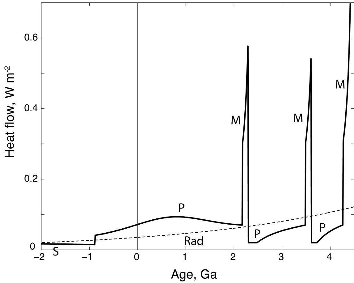
Figure 2 The heat flow as a function of age for the nonmonotonic model (dark line) and the radioactive heat generation as heat flow (thin dashed line). The modes of convection are (M) mush ocean, (P) plates, and (S) stagnant lid.
