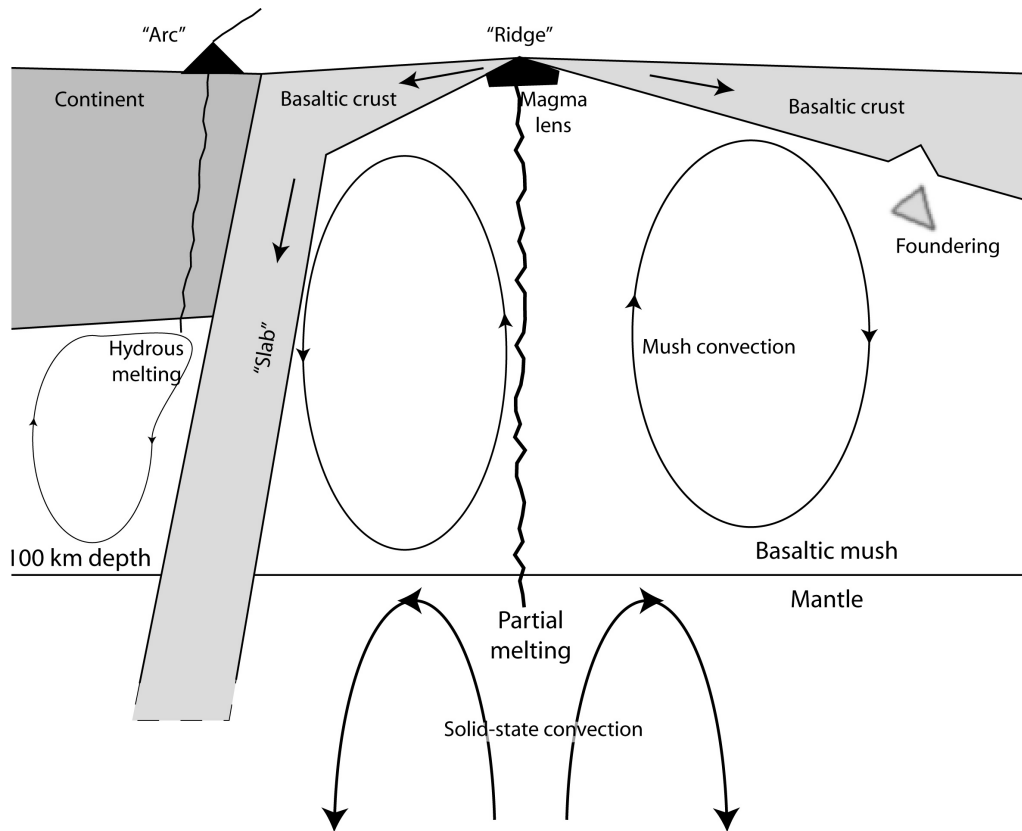
Figure 7 Schematic diagram of mush ocean with vertical exaggeration. Analogues to plate tectonic features are in quotes. Upwelling mantle partially melts. Melt ascends into the magma lens at the ridge axis and freezes, making basaltic crust and basaltic mush. Basaltic crust both subducts as slabs and founders as blocks. Partial melting of hydrated basalt produces arcs and continents. Convection within the mush transfers additional heat from the mantle. Slabs, entrained mush, and foundered blocks return basaltic material to the mantle. Thick lithosphere composed of depleted mantle residuum stabilized some continental regions (not shown).
