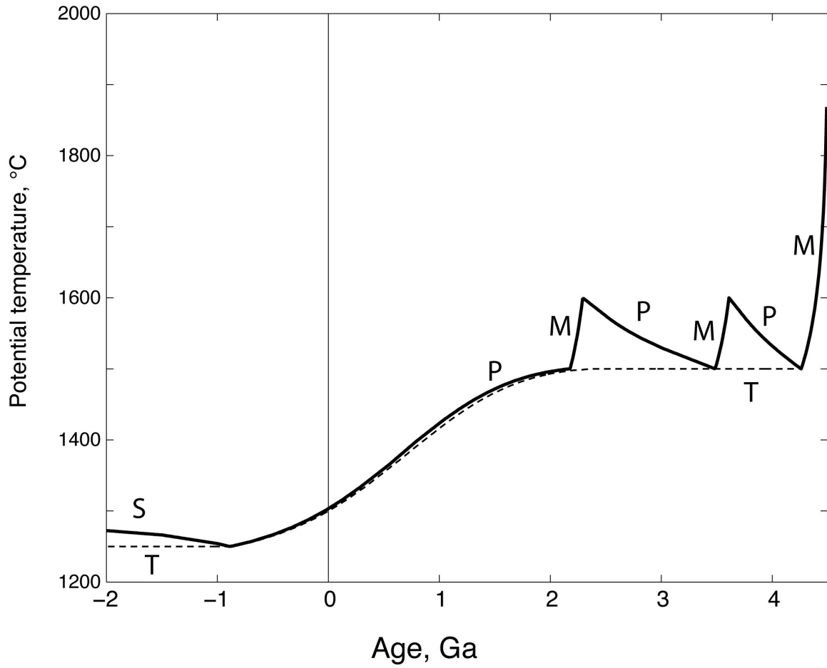
Figure 3 The thermal history for the nonmonotonic model (dark line) and the monotonic model (thin dashed line). The modes of convection are (M) mush ocean, (P) plates, (S) stagnant lid, and (T) transition in the monotonic model. The temperature remains constant in the transitions in the monotonic model.
