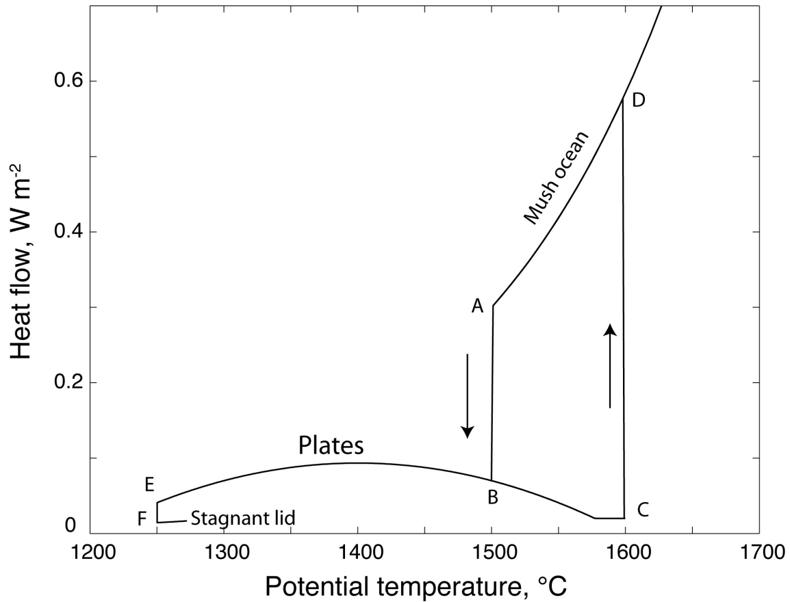
Figure 1 Assumed heat flow from the Earth's mantle as a function of the potential temperature of the Earth's interior. The model starts a 2000°C at 4.5 Ga. The mantle cools along the mush ocean path until it reaches point A. The nonmonotonic model jumps to plate tectonics at point B. If the heat flow is less than the radioactive heat generation the mantle cools along the plate branch moving toward point E. If the heat flow is lower than radioactive heat generation the mantle heats up to point C, where convection jumps to the mush ocean branch at point D. It then cools to point A. The nonmonotonic model jumps to stagnant lid convection from point E to F. The mantle then heats up. The monotonic model stays at the jumps with the heat flow equal to radioactive heat generation until radioactive heat generation decreases to heat flow of the cooler mode. Note Thom (1983) popularized this presentation method in his catastrophe theory. I eschew the word "catastrophe" in the text as it is preempted with a foul stench in the Earth sciences. One could add another axis perpendicular to the plane of the diagram. Continental area would be a good choice ( Lenardic et al. , 2005). One would then need the net growth (shrinkage) age of continents as a function of interior temperature, convection mode, and continental area to compute forward modes.
