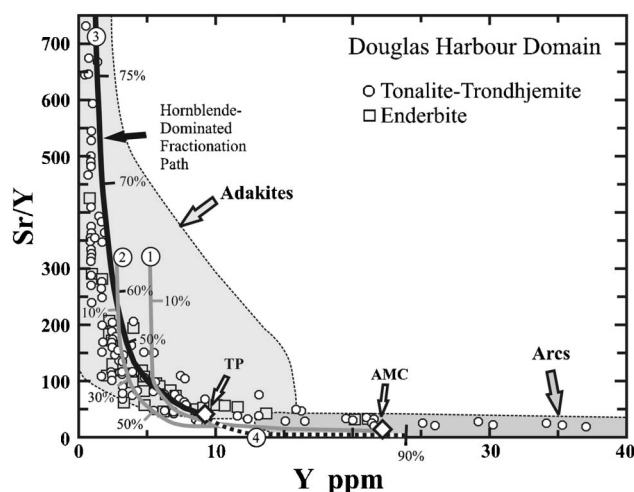
Fig. 4. Sr/Y vs. Y diagram showing the distribution of tonalites, trondhjemites and enderbites (pyroxene-tonalites) from the Douglas Harbour Domain (Minto Block, NE Superior Province). Thick grey curves show the distribution of batch melts derived from an Archaean Mafic Composite (AMC) source (Drummond and Defant, 1990) in equilibrium with eclogite (1) and garnet amphibolite (10% gt, 2) restite assemblages. The Adakite and Arc fields are from Castillo et al. (1999). The heavy black curve (3) is a hornblende-dominated fractional crystallization path from a tonalitic parental melt (TP). The dotted black curve (4) shows a fractionation path for up to 90% dioritic fractionation (50:50 hornblende + plagioclase). Both fractionation models (3 and 4) were calculated using the constant D values shown in Table 1.
