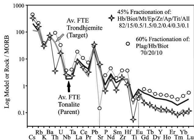
Fig. 7. Multi-element trace element profiles normalized to normal MORB (mid-ocean-ridge basalt: Sun and McDonough, 1989) for average tonalite and trondhjemite from the Eastern Faribault-Thury Complex. Two fractionation models are shown. The circles + dotted line shows results of 60% fractionation of a plagioclase + hornblende + biotite assemblage, while the stars with filled line show results for 45% hornblende-dominated fractionation. Plag, plagioclase; Hb, hornblende; Biot, biotite; Mt, magnetite; Ep, epidote; Zr, zircon; Ap, apatite; Tit, titanite; All, allanite. The prominent negative Th anomaly is caused by the extremely high D for Th in allanite. It is possible that in nature, allanite crystals may not be able to scavenge enough Th from the surrounding melt to satisfy its appetite for this element. The very large negative Ti anomaly results from use of an hornblende/melt D_{\text{Ti}} value of c. 4. Although this value seems appropriate for melts of 60% \text{SiO}_2 (Fig. 6), there is considerable scatter, and the value applicable to TTG differentiation could be somewhat lower.
