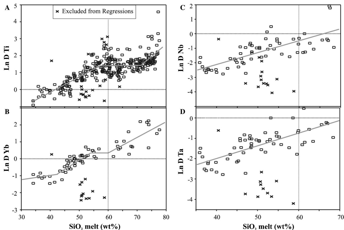
Fig. 6. Example of methodology used to parameterize D -data, shown here for Ti, Yb, Nb, and Ta in amphibole, using data from the literature. The complete REE profile at 60% \text{SiO}_2 was smoothed using the Lattice Strain Model of Blundy and Wood (1994), and results are given in Table 1.
