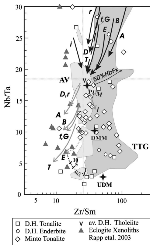
Fig. 9. Nb/Ta vs. Log(Zr/Sm) diagram adapted from Rapp et al. (2003). The grey TTG field and eclogite xenoliths are from Rapp et al. (2003). The pale grey field labeled AV is the field of Superior Province Archaean mafic volcanics from Rapp et al. (2003), complemented by data from the Douglas Harbour Domain (Madore et al., 1999). The open symbols show tonalites and mela-enderbites ( \text{SiO}_2 < 70\% ) from the Douglas Harbour domain (D.H.) and other Minto locales (Bédard, 2003). Note that these data extend offscale to higher Nb/Ta than shown here. The intersecting dashed lines show chondritic ratios, while the star marked 'PUM' is primitive upper mantle (Sun and McDonough, 1989). The star marked 'DMM' is depleted MORB mantle from Workman and Hart (2005), while the star marked 'UDM' is for ultra-depleted mantle from Bédard (1999) residual from c. 25% melting of PUM, which is used in the model shown in Fig. 13. The 'v' is the average metabasalt used in the modeling of Fig. 8. The bold black arrows show the melt trends (% melting increasing from 5 to 40%), produced in the different equilibrium melting models, while the grey arrows show the trend of the corresponding restites. Restite assemblages are: A: 100% Hb; B: 65:15:20 Cpx:Hb:Gt; D: 80:19:1 Cpx:Gt:Rut; E: 80:20 Cpx:Gt; f: 98.9:1:0.1 Cpx:Gt:Rut; G: 20:20:60 Cpx:Opx:Pg; r: 41.5:38:20:0.5 Cpx:Opx:Gt:Rut; T: 18:77:3:2 Cpx:Opx:Gt: Titanite; i: 20:71:4:5 Cpx:Opx:Gt: ilmenite. Hb, Hornblende; Cpx, Clinopyroxene; Opx, Orthopyroxene; Pg, Plagioclase; Rut, Rutile; Gt, Garnet. The arrow trending to the top right labeled 50% HbF shows the path of 50% fractionation of an hornblende-dominated assemblage (Fig. 7) from the EFT tonalite parent. The dotted line labelled 'MIX' at the bottom of the figure shows results of mixing residues of 40% crustal anatexis (curve 'E') with the ultra-depleted mantle residue (UDM). The numbers represent the % of crustal restite in the mixture.
