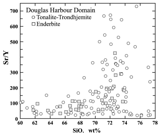
Fig. 5. Sr/Y vs. \text{SiO}_2 diagram showing tonalites, trondhjemites, and enderbites (pyroxene-tonalites) from the Douglas Harbour Domain. Note the overall trend of increasing Sr/Y as \text{SiO}_2 increases.
