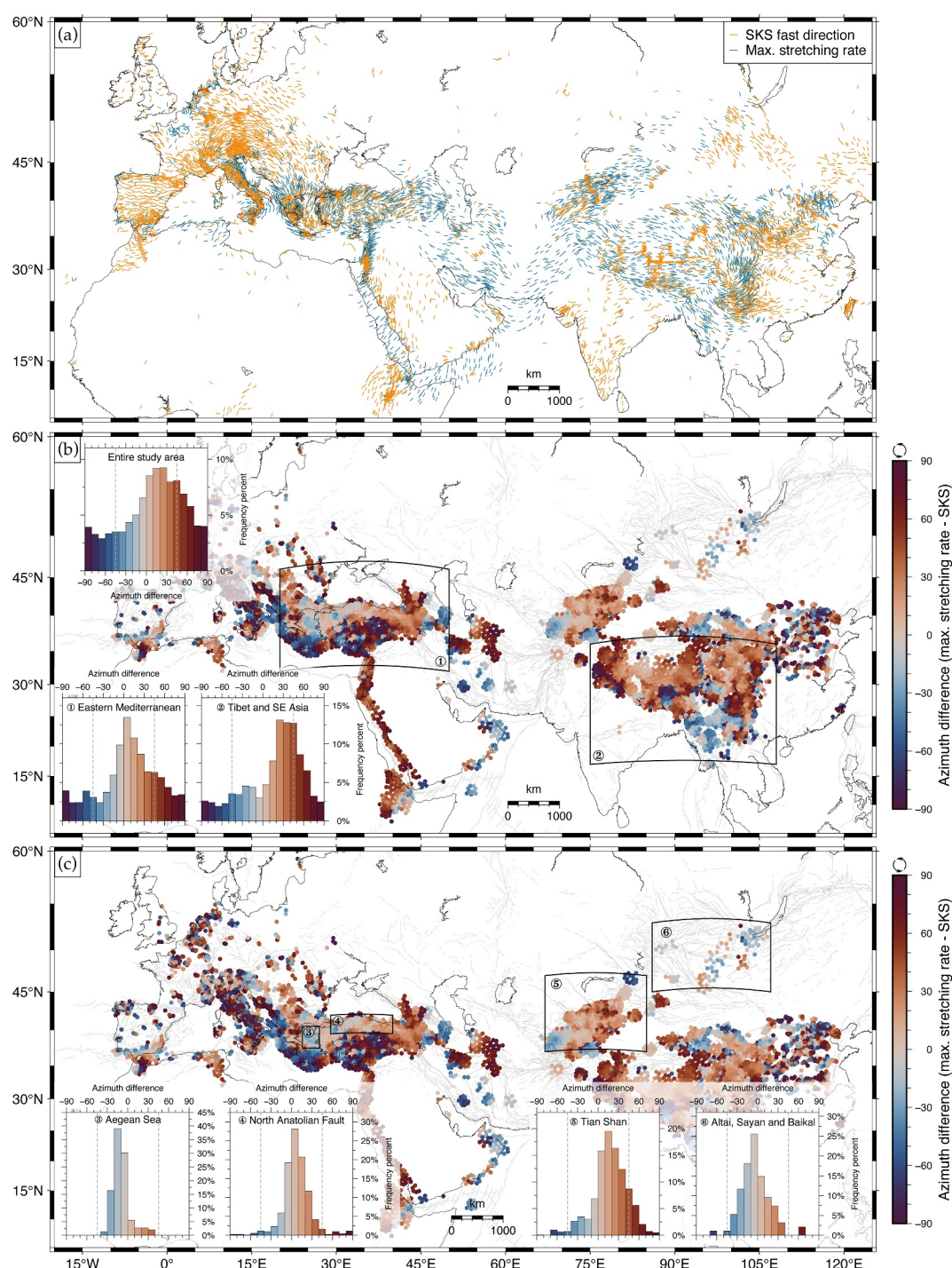
Figure 10. (a) GNSS-derived maximum stretching rate azimuths \hat{\epsilon}_1 (blue) and SKS fast orientations (orange), compiled by Becker et al. (2012, updated 02/2025). (b, c) Signed azimuthal differences between \hat{\epsilon}_1 and SKS fast orientations, with histograms showing distributions across the Alpe Belt (top-left) and in selected regions: (1) eastern Mediterranean, (2) Tibet and SE Asia, (3) Aegean Sea, (4) North Anatolian fault, (5) Tian Shan, and (6) Altai-Sayan-Baikal regions. Dashed vertical gray lines mark maximum shear strain rate directions ( \pm 45^\circ from \hat{\epsilon}_1, \hat{\epsilon}_2 ). Warm colors indicate clockwise offsets of \hat{\epsilon}_1 relative to fast SKS directions, cool colors counter-clockwise, and dark purple near-perpendicular orientations. A mask was applied to show only regions where strain rates exceed 10 nanostrain/yr.
