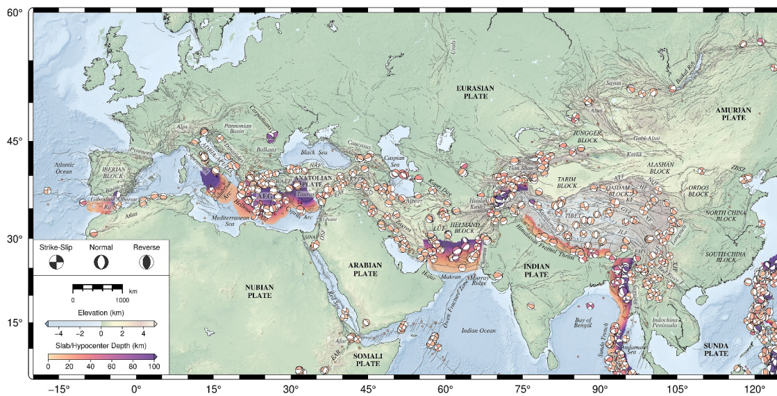
Figure 1. Main tectonic features and seismicity along the Alpine-Himalayan belt. Slab depths are from Slab2 (Hayes et al., 2018) and ESHM2020 (Danciu et al., 2024). Faults are sourced from AFEAD (Zelenin et al., 2021). Moment tensors for M_W \geq 6 earthquakes are from the gCMT catalog (Dziewonski et al., 1981; Ekström et al., 2012), with 6 \geq M_W \geq 5 earthquakes represented as dots. AEG, Aegean Sea plate; WAEP, Western Anatolian Extensional Province; DSF, Dead Sea Fault; EAF, East Anatolian Fault; NAF, North Anatolian Fault; EAR, East African Rift; ATF, Altyn Tagh Fault; KF, Kunlun Fault; EHS, Eastern Himalayan Syntaxis; XJF, Xiaojiang Fault; XF, Xianshuihe Fault; JF, Jiali Fault; GYF, Ganzi-Yushu Fault; ZBSZ, Zhangjiakou-Bohai Seismic Zone; LJF, Lijiang Fault; HF, Haiyuan Fault; NQF, North Qilian Fault.
