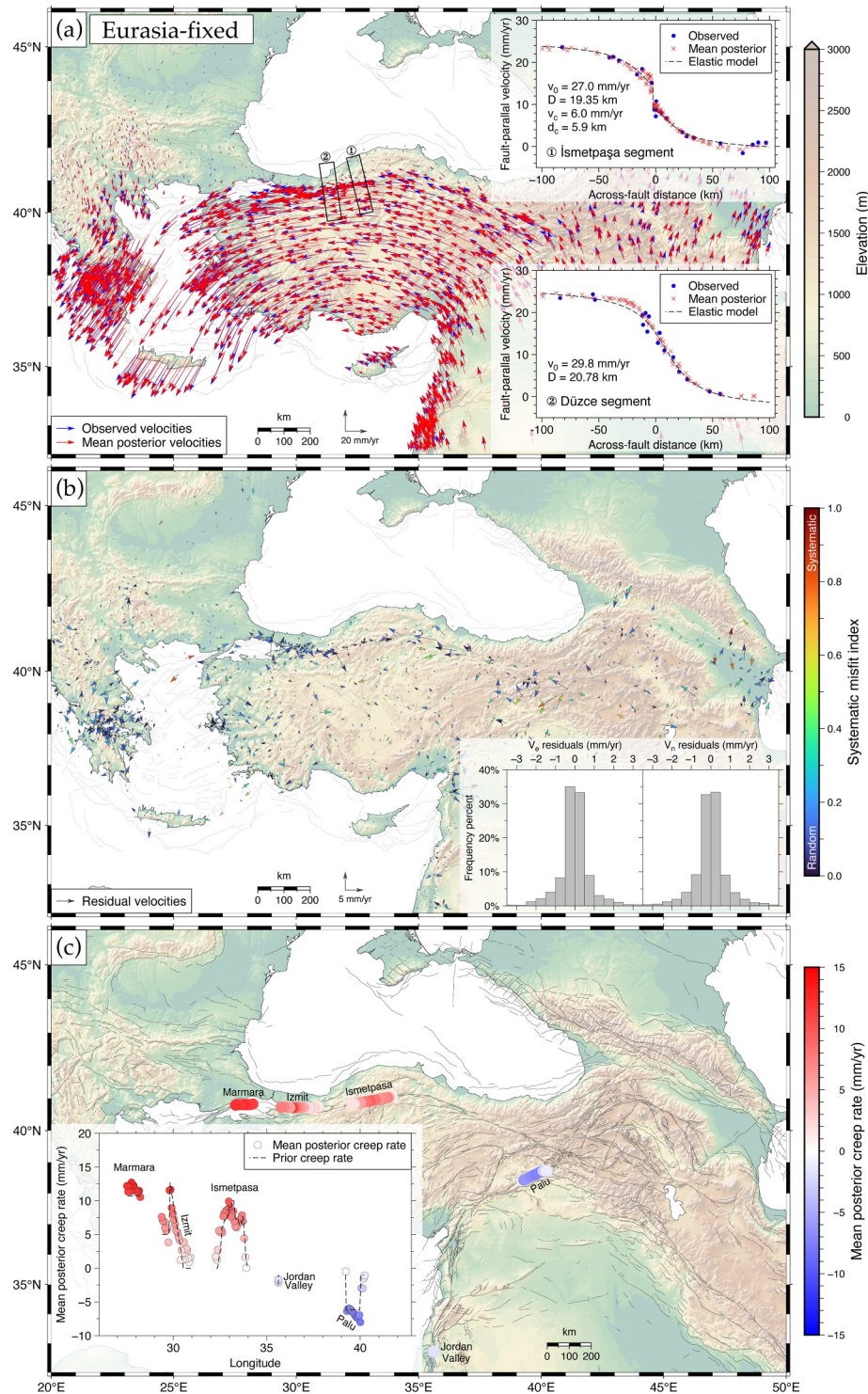
Figure 6. (a) Comparison of observed velocities (blue vectors) and mean posterior velocities (red vectors). Profiles 1 and 2 show observed, mean posterior, and screw-dislocation model-predicted velocities (Savage & Burford, 1973; Weertman & Weertman, 1964) across the İsmetpaşa and Düzce segments of the North Anatolian Fault. Profiles demonstrate accurate modeling of velocity gradients—even across creeping faults—when dense near-fault GNSS velocities are available. (b) Residual velocities (observed minus modeled) colored by their systematic misfit index (red: systematic, blue: random). Histograms show the distribution of east and north velocity residuals. (c) Mean posterior creep rates on select fault segments (red: right-lateral creep rates, blue: left-lateral creep rates), with a profile showing prior and mean posterior creep rate variability along select fault segments as a function of longitude.
